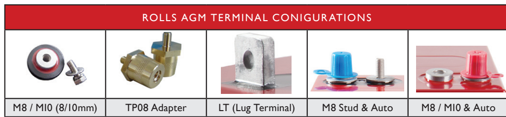
Terminal Connections for AGM-S & AGM-R models.
